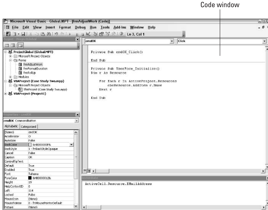
Figure 25-22: The Code window for the UserForm allows you to add VBA code that will run when the user clicks the OK button.
