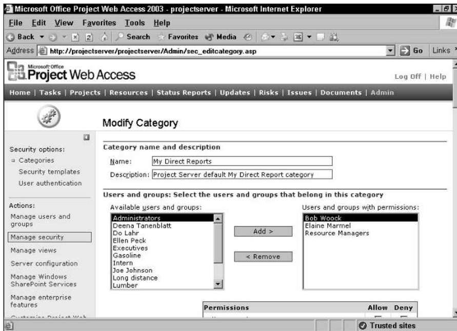
Figure 19-14: Use this page to define the users that you want to include in the category.
