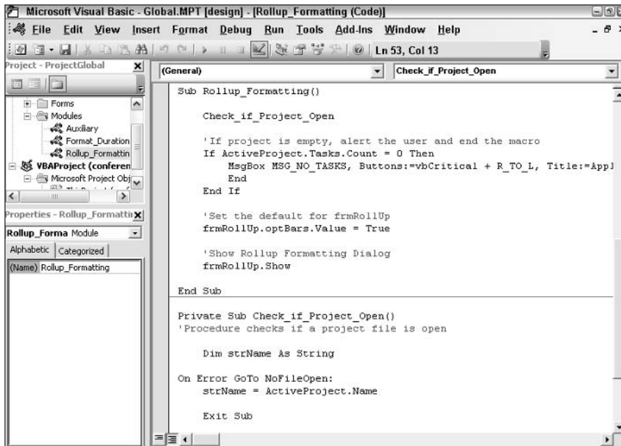
Figure 24-1: A sample set of instructions that are stored in a macro.
