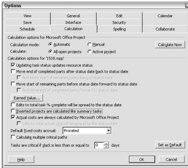
Figure 15-20: The Inserted projects are calculated like summary tasks check box controls whether Project uses the subprojects' late finish dates or the master project's late finish date for calculations.
