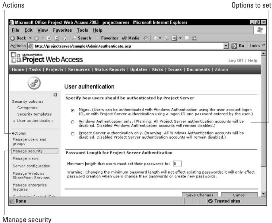
Figure 19-4: Control authentication and password issues from this page.
