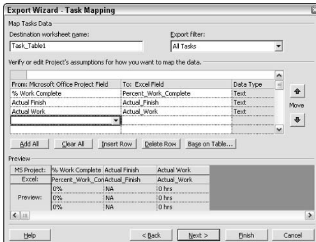
Figure 26-3: As you add fields in the Task Mapping dialog box, a preview of the Excel worksheet that you're creating appears at the bottom of the Task Mapping dialog box.
