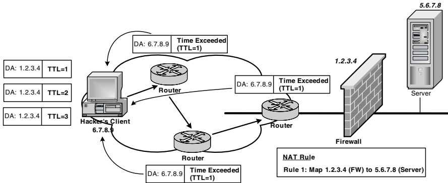
Exhibit 10. Traceroute Operation
