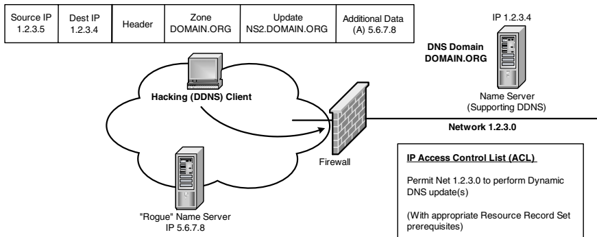
Exhibit 12. DDNS Spoofing
