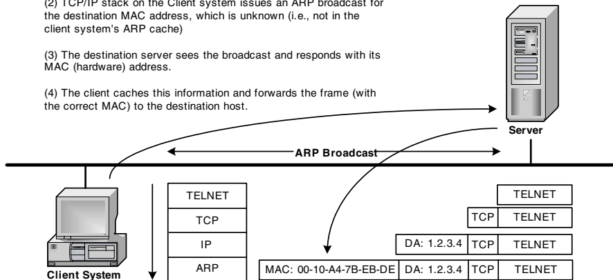
Exhibit 2. ARP Resolution
