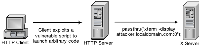
Exhibit 42. X-Term Exploit
