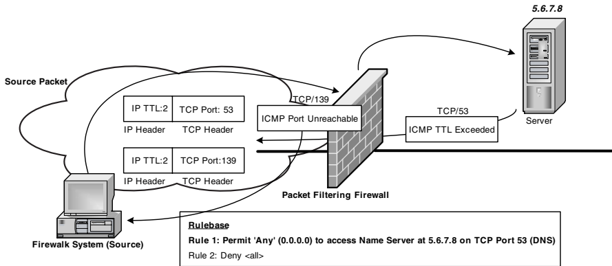
Exhibit 8. Firewalk against Packet Filtering Firewall
