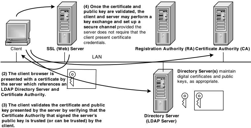
Exhibit 25. Public Key Infrastructure Authentication
