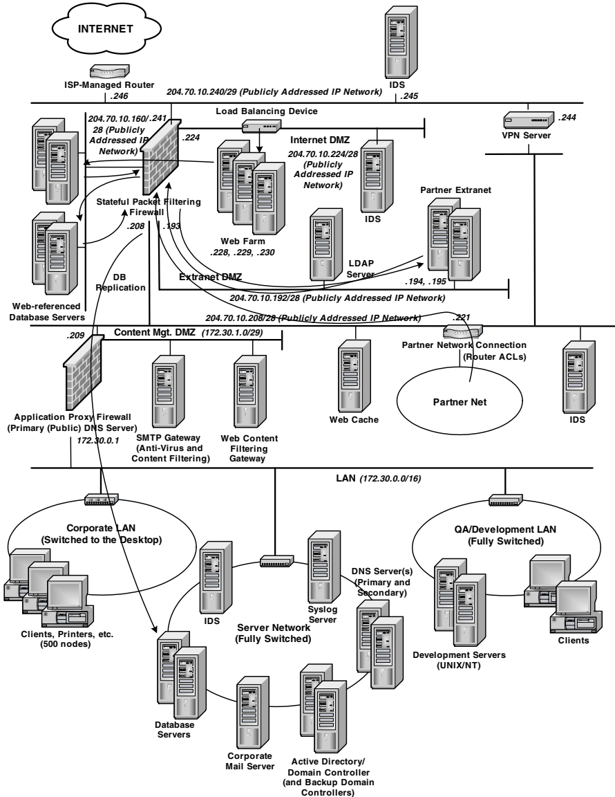
Exhibit 4. Updated Network Diagram
