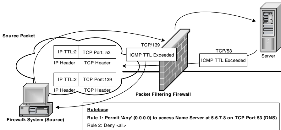
Exhibit 12. Firewalk against Packet Filtering Firewall
