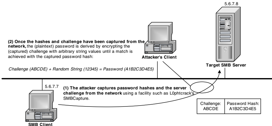
Exhibit 3. SMBCapture
