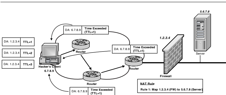
Exhibit 17. Traceroute Operation
