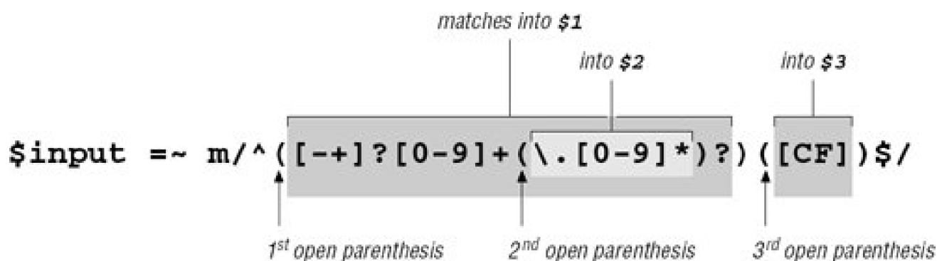
Figure 2-3. Nesting parentheses
