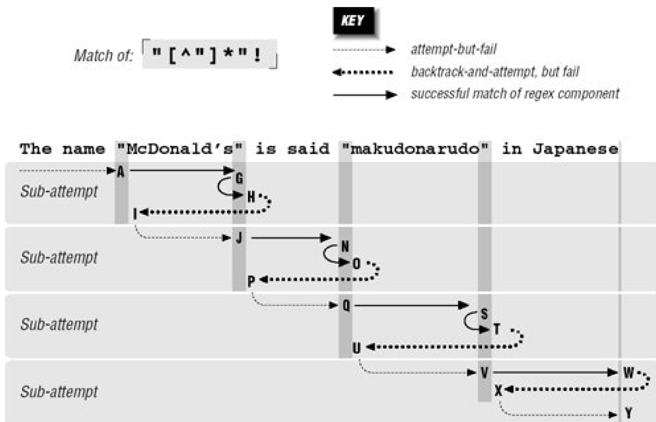
Figure 6-5. Failing attempt to match "[^"]*"
