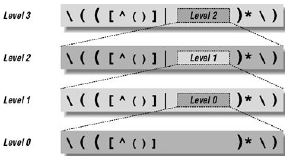
Figure 7-1. Matching a few levels of parentheses
