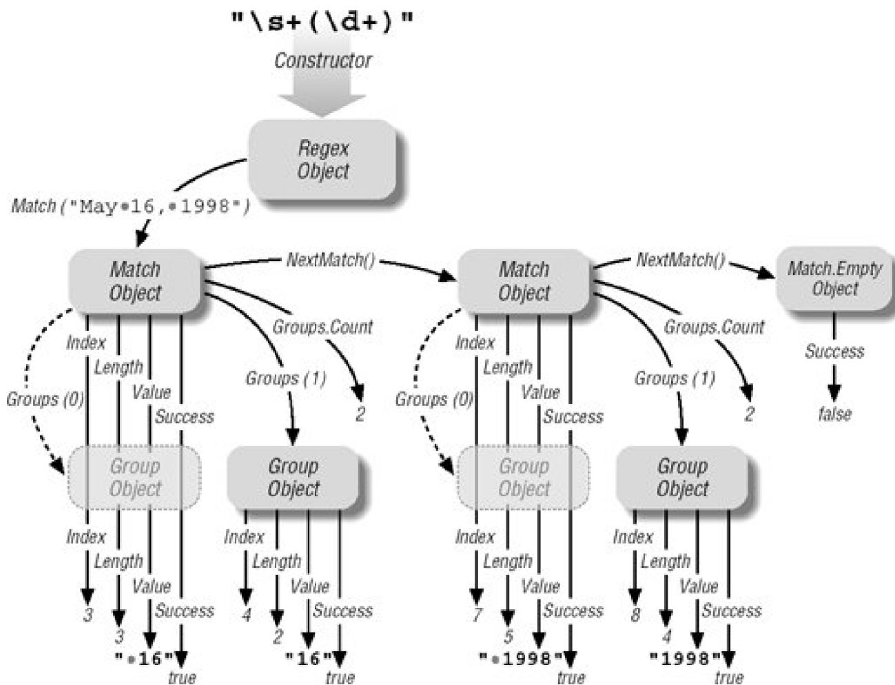
Figure 9-1. .NET's Regex-related object model
