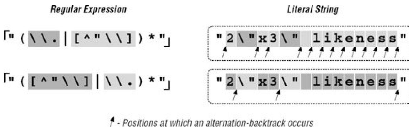
Figure 6-1. Effects of alternative order (Traditional NFA)
