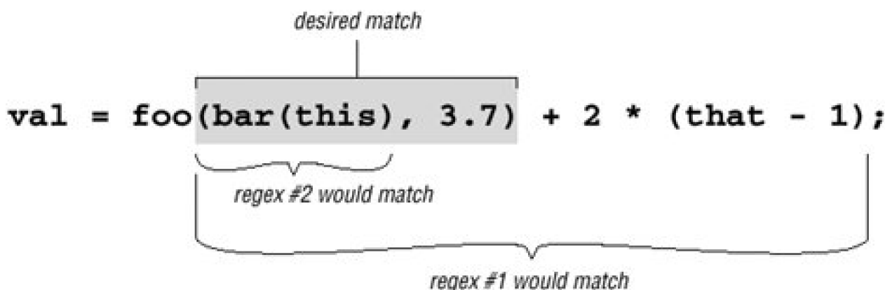
Figure 5-1. Match locations of our sample regexes
