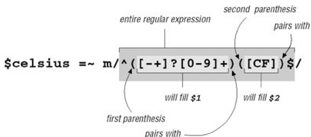
Figure 2-1. Capturing parentheses
