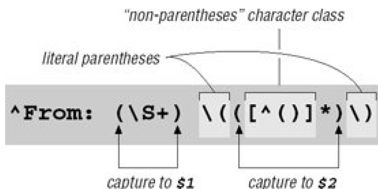
Figure 2-4. Nested parentheses; $1, and $2
