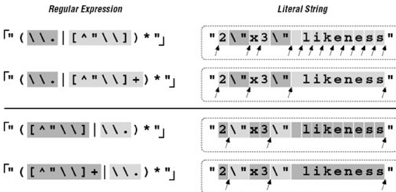
Figure 6-2. Effects of an added plus (Traditional NFA)
