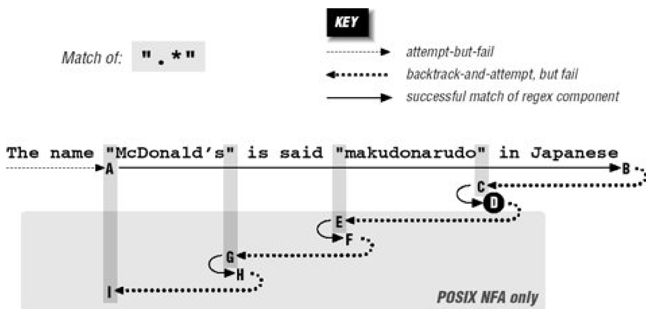
Figure 6-3. Successful match of " .* "
