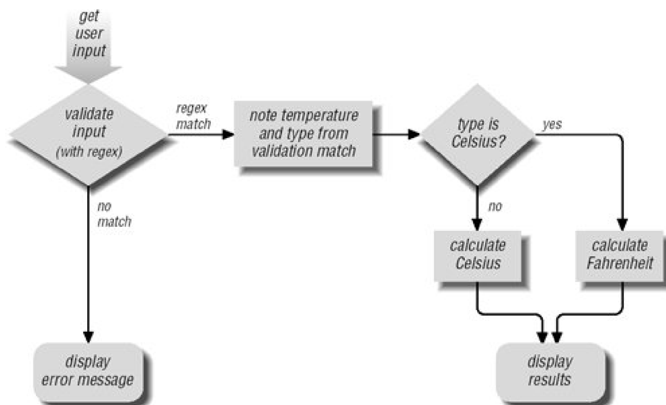
Figure 2-2. Temperature-conversion program's logic flow
