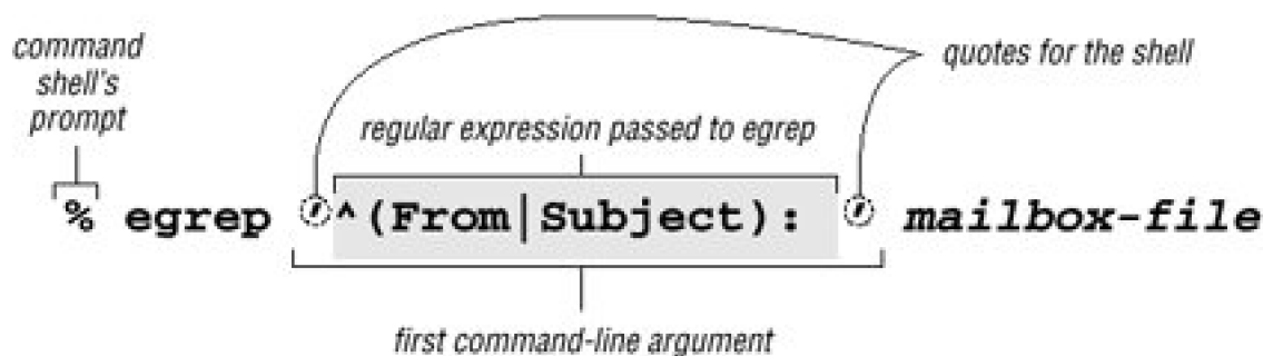
Figure 1-1. Invoking egrep from the command line
