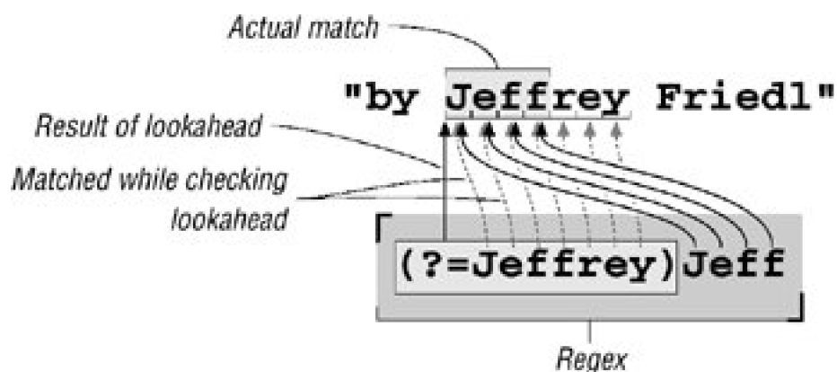
Figure 2-5. How (?=Jeffery)Jeff is applied
