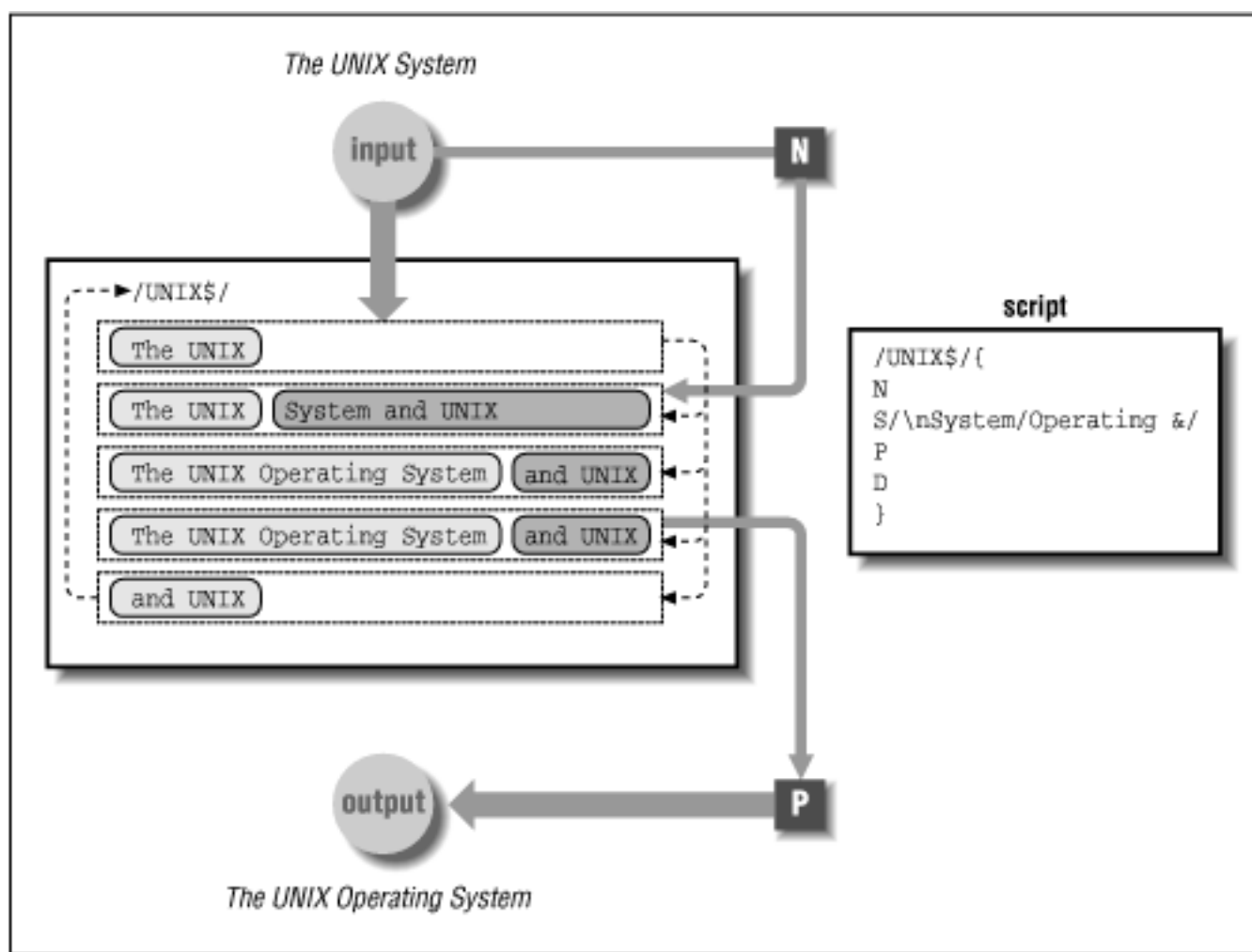
Figure 6.1: The Next, Print, and Delete commands used to set up an input/output loop
