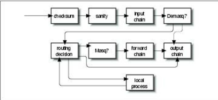
Figure 9-8. Datagram processing chain in IP chains
