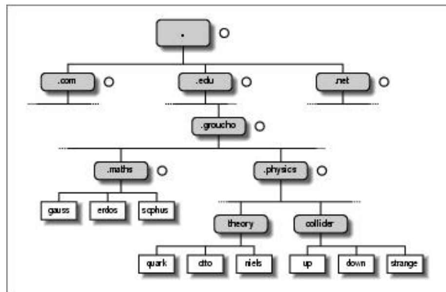
Figure 6-1. A part of the domain namespace
