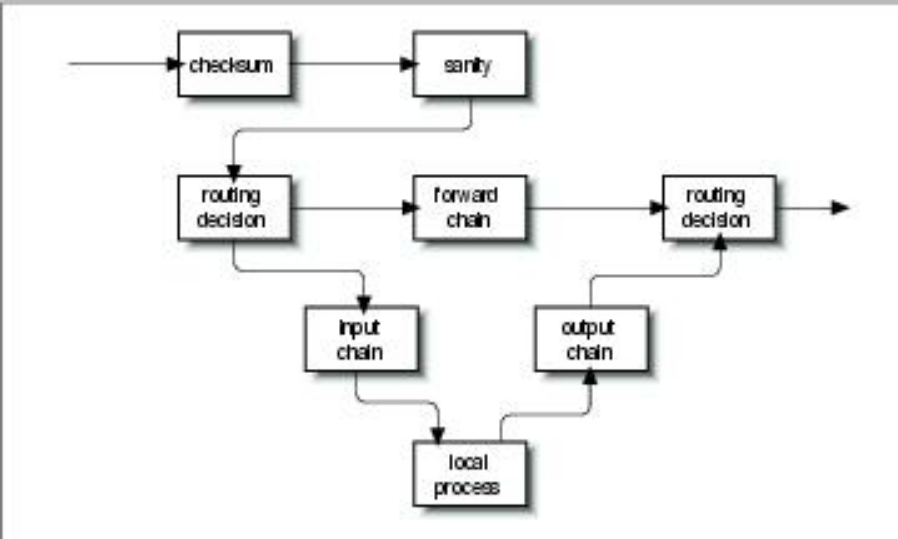
Figure 9-9. Datagram processing chain in netfilter
